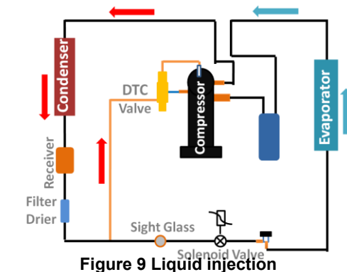
Figure 9 Liquid injection
