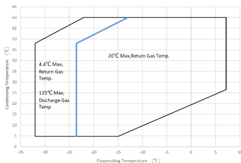
Figure 2 Envelop for R454C/R454A/R455A
