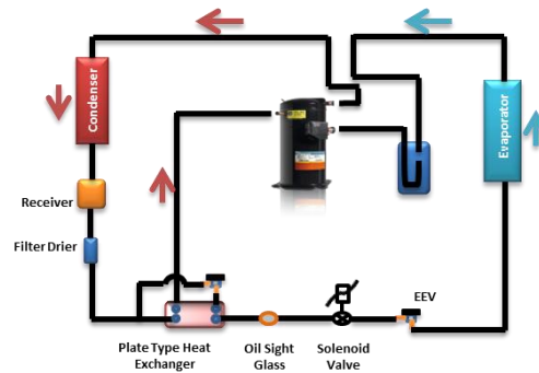
Figure 10 Vapor injection
