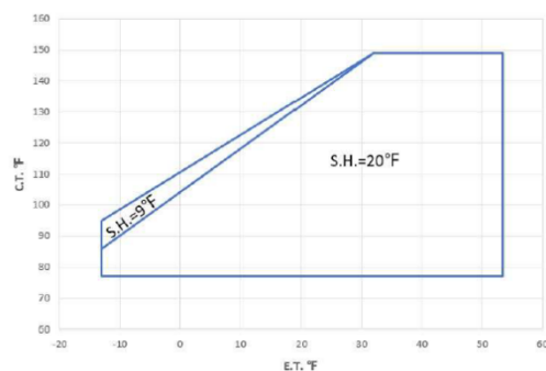
Figure 2 Envelop for R454B
